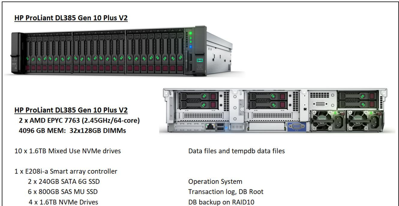
Figure 0.1 Benchmark and priced configuration for HPE ProLiant DL385 Gen10 Plus V2
