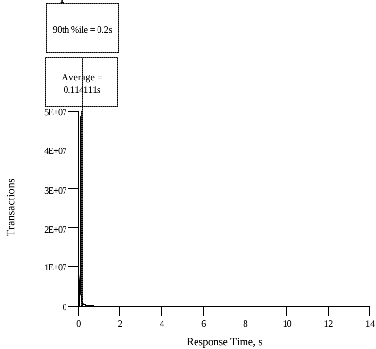
Figure 6.1: New Order Response Time Distribution
