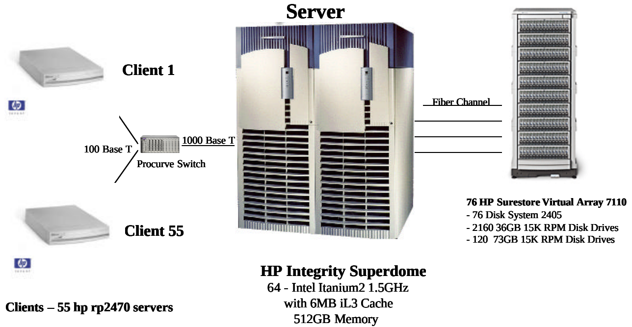
Figure 1.1: HP Integrity Superdome Priced Configuration
