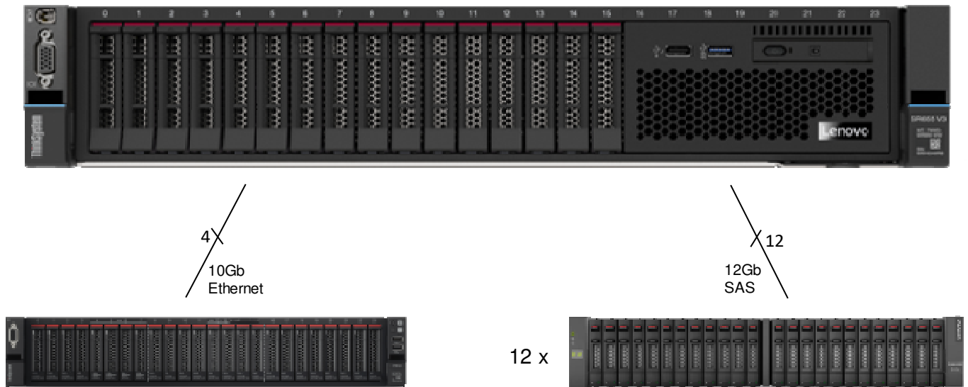
Figure 1-1. Measured Configuration
