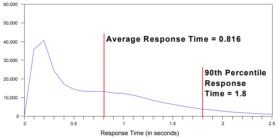
Figure 6. iSeries 400 Model 840-2420 Stock-Level Response Time Distribution
