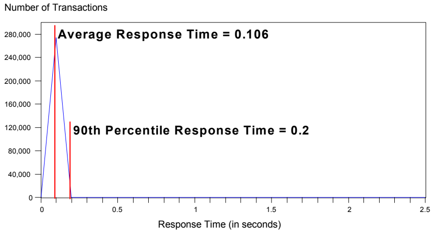
Figure 4. iSeries 400 Model 840-2420 Delivery (Interactive) Response Time Distribution
